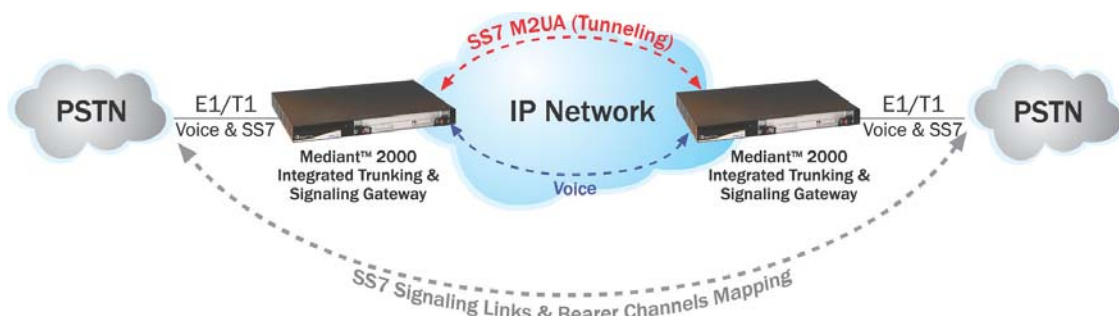
Figure 3: TDM & SS7 Tunneling Architecture
