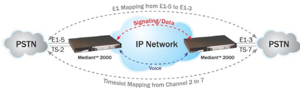
Figure 3: TDM & SS7 Tunneling Architecture
